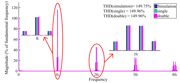
FIGURE 12. The harmonic spectrum in the case of pure resistance.
