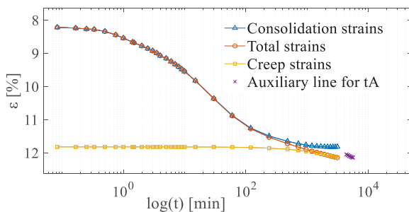
Fig. 7. Oedometer step filtered in ANACONDA.
