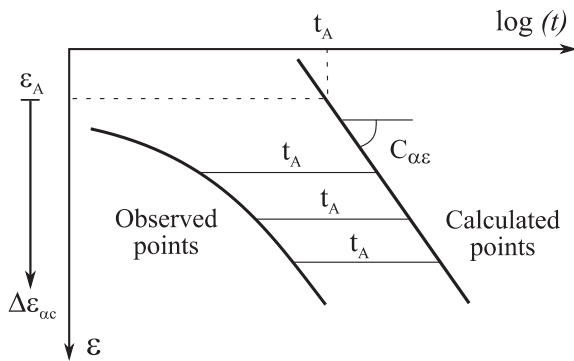
Fig. 6. Observed creep points and the auxiliary straight line.
