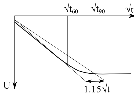
Fig. 3. Construction of the square root of time fitting method.
