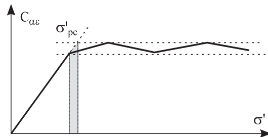
Fig. 8. Akai uses C_{\alpha\varepsilon} to determine preconsolidation stress.
