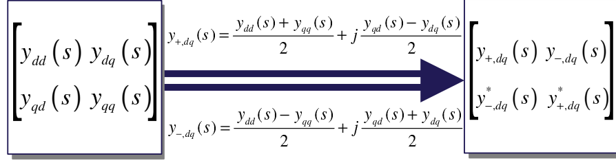
Fig. 3. The complex transfer function equivalent of an asymmetric transfer function matrix.
