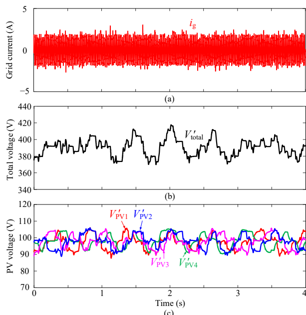
Fig. 19. Performance of the random sampling-rate MPPT method operated at 100 W/m 2 and 25 °C: (a) grid current, (b) the equivalent total DC voltage, and (c) filtered PV voltages.
