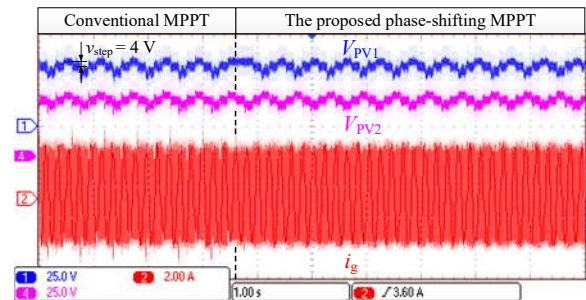
Fig. 23. Experimental results of the PS-MPPT on a 2-cell CHB PV inverter, operated at 200 \text{ W/m}^2 and 25 \text{ }^\circ\text{C} , with the PV rated power being 300 W for each cell, and the grid voltage is 40 V(rms) ( V_{PV1} [25 V/div] and V_{PV2} [25 V/div]; DC voltages for cell #1 and #2; i_g [2 A/div]; grid current).
