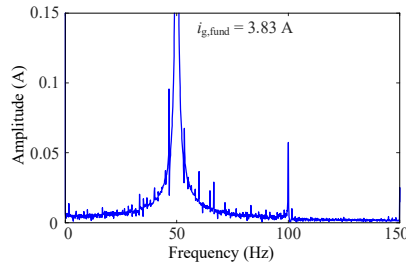
Fig. 26. FFT analysis of the grid current i_g shown in Fig. 25.
