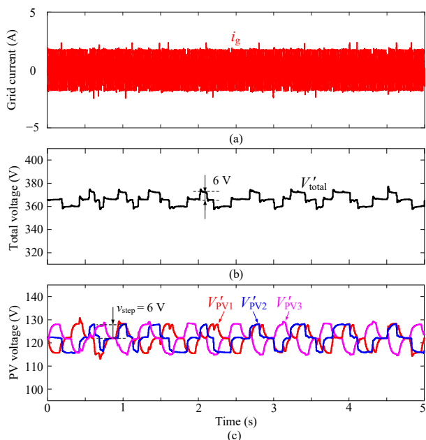
Fig. 17. Performance of the hybrid PS-MPPT method operated at 100 W/m 2 and 25 °C: (a) grid current, (b) the equivalent total DC voltage, and (c) filtered PV voltages.
