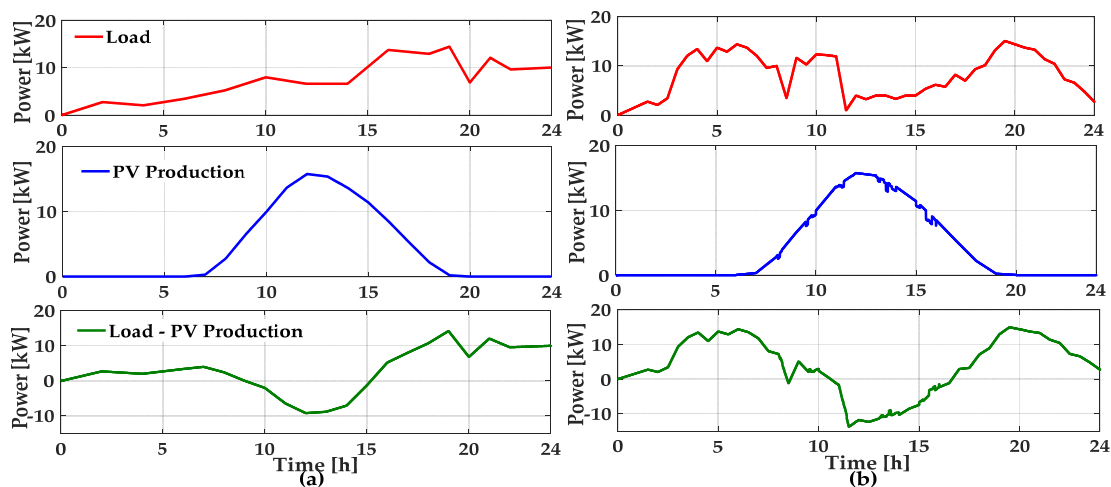
Figure 9. Total load, PV production and (total load - PV production). (a): without passing clouds and (b): with passing clouds. A day in May was used as a case study.
