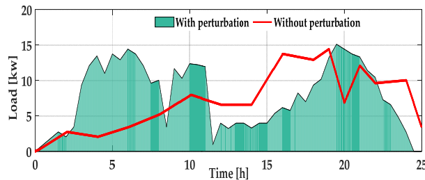
Figure 5. Load profiles.
