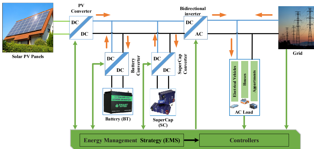
Figure 1. Overall microgrid architecture.
