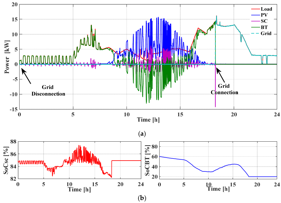
Figure 14. EEMS-with passing clouds, A day in May December used as a case study: (a) powers; (b) the SoCs.
