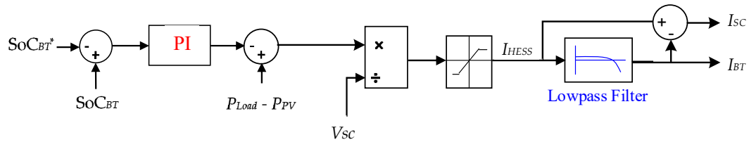
Figure 6. Energy management scheme: classical PI control.
