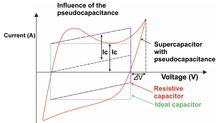
Figure 4. SC characteristics.
