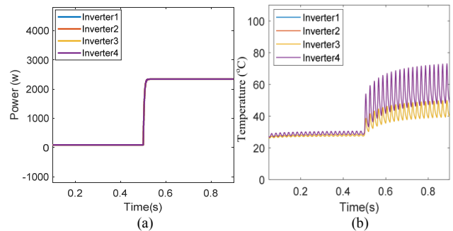
Fig. 11. Simulated results of 4 paralleled inverters with parameters shown in TableI. (a) Active power sharing of inverters. (b) Power device junction temperature of inverters.
