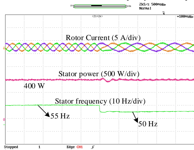
Fig. 9. Step response of stator frequency change.
