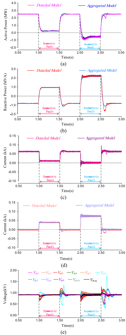
FIGURE 11. Simulation results of detailed model and aggregated model under the condition of grid faults with weak grid circumstance. (a) active power curve; (b) reactive power curve; (c) d-axis current; (d) q-axis current; (e) dc-link voltages of front-end circuit.
