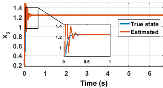
Fig. 11. Estimation of x_2 using Quasi-Luenberger observer.
