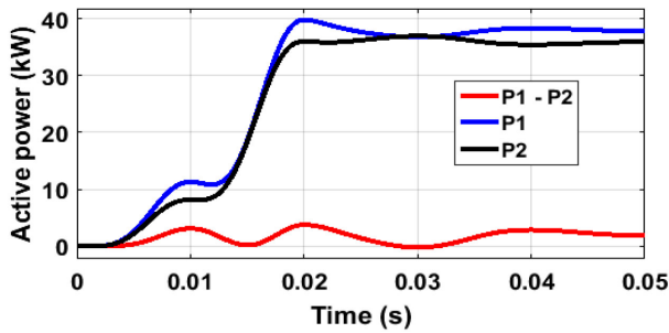
Fig. 20. Active powers of two ILCs.
