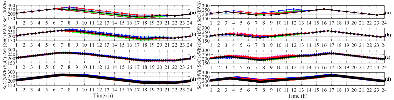
Fig. 4. Numerical stability test demonstrated by convergence of the results for the EES SoC for the summer (left) and winter (right), for \Delta t = 60, 30, 15, and 1 minutes in (a), (b), (c) and (d) respectively.
