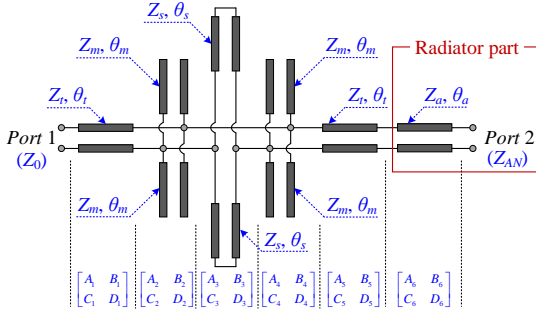
Fig. 2. Equivalent circuit of the proposed filtering antenna.
