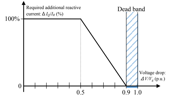
(b) Additional reactive current requirement during LVRT
