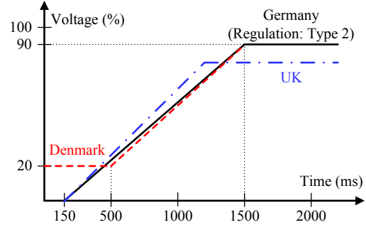
(a) LVRT requirement by different countries.
