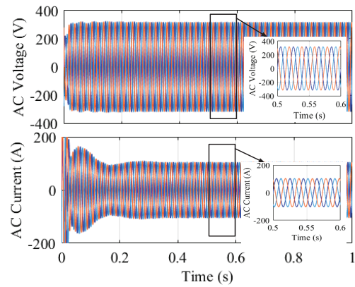
Fig. 15: The three-phase ac voltage/current waveform under L_g = 0.58\text{mH} .
