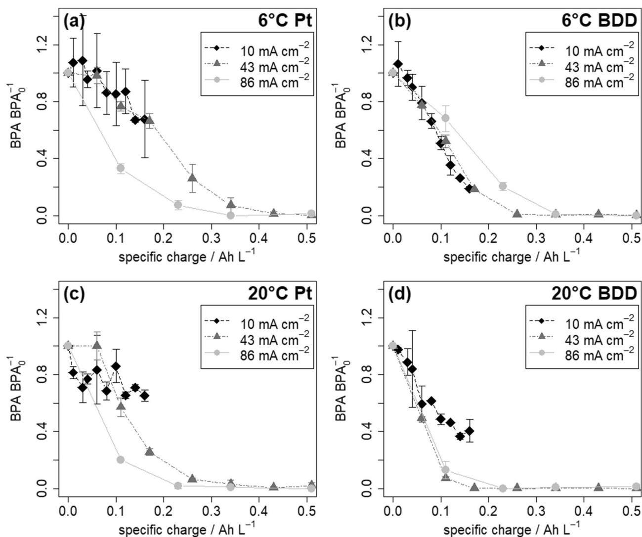
Fig. 2 Degradation of BPA in LL vs specific charge ( \text{Ah L}^{-1} ) until complete removal or maximal experimental time was reached: a Pt and 6 °C, b BDD and 6 °C, c Pt and 20 °C, d BDD and 20 °C; Error bars indicate the standard deviation of the two replicate experiments
