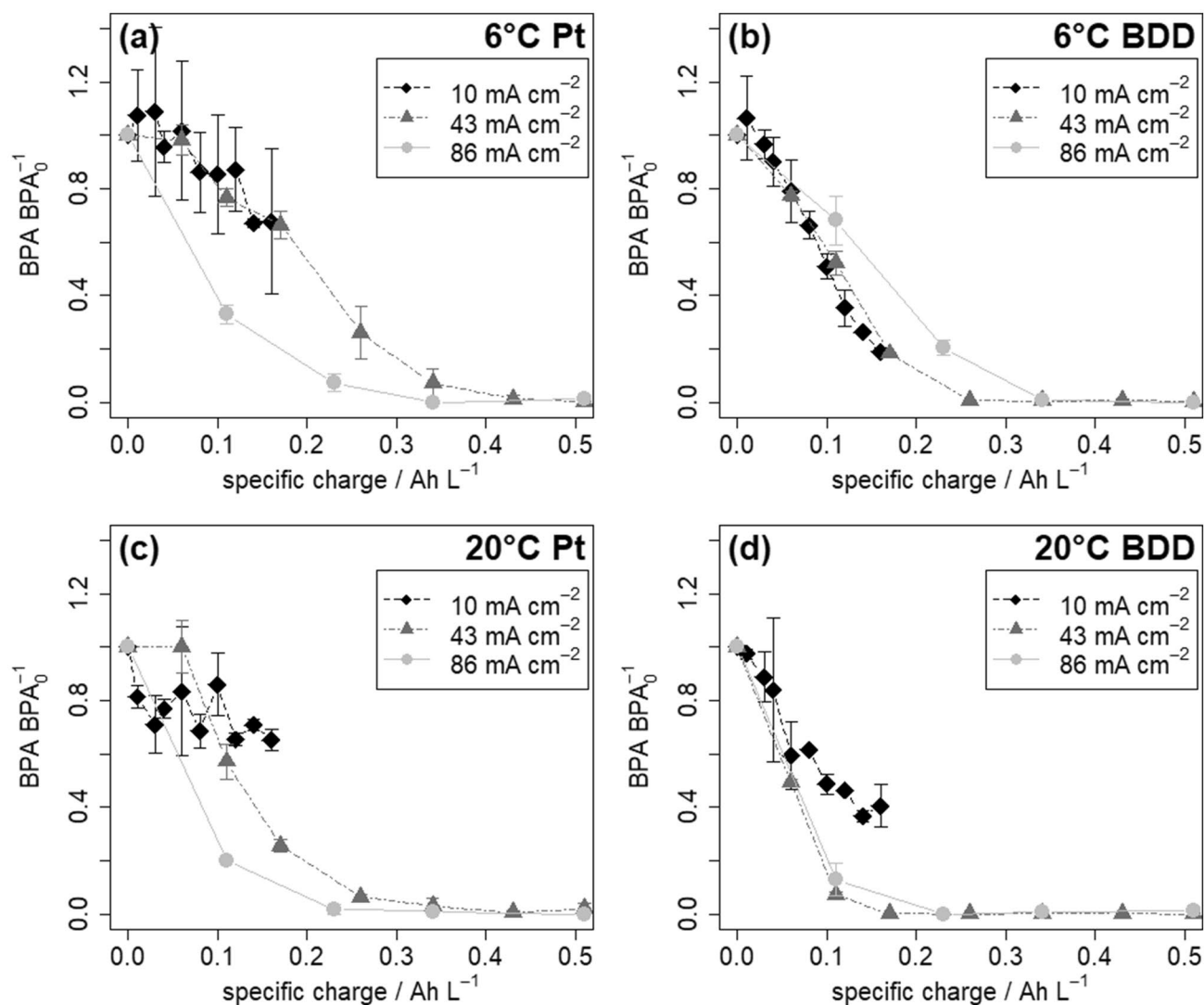
Fig. 2 Degradation of BPA in LL vs specific charge ( \text{Ah L}^{-1} ) until complete removal or maximal experimental time was reached: a Pt and 6\text{ }^{\circ}\text{C} , b BDD and 6\text{ }^{\circ}\text{C} , c Pt and 20\text{ }^{\circ}\text{C} , d BDD and 20\text{ }^{\circ}\text{C} ; Error bars indicate the standard deviation of the two replicate experiments
