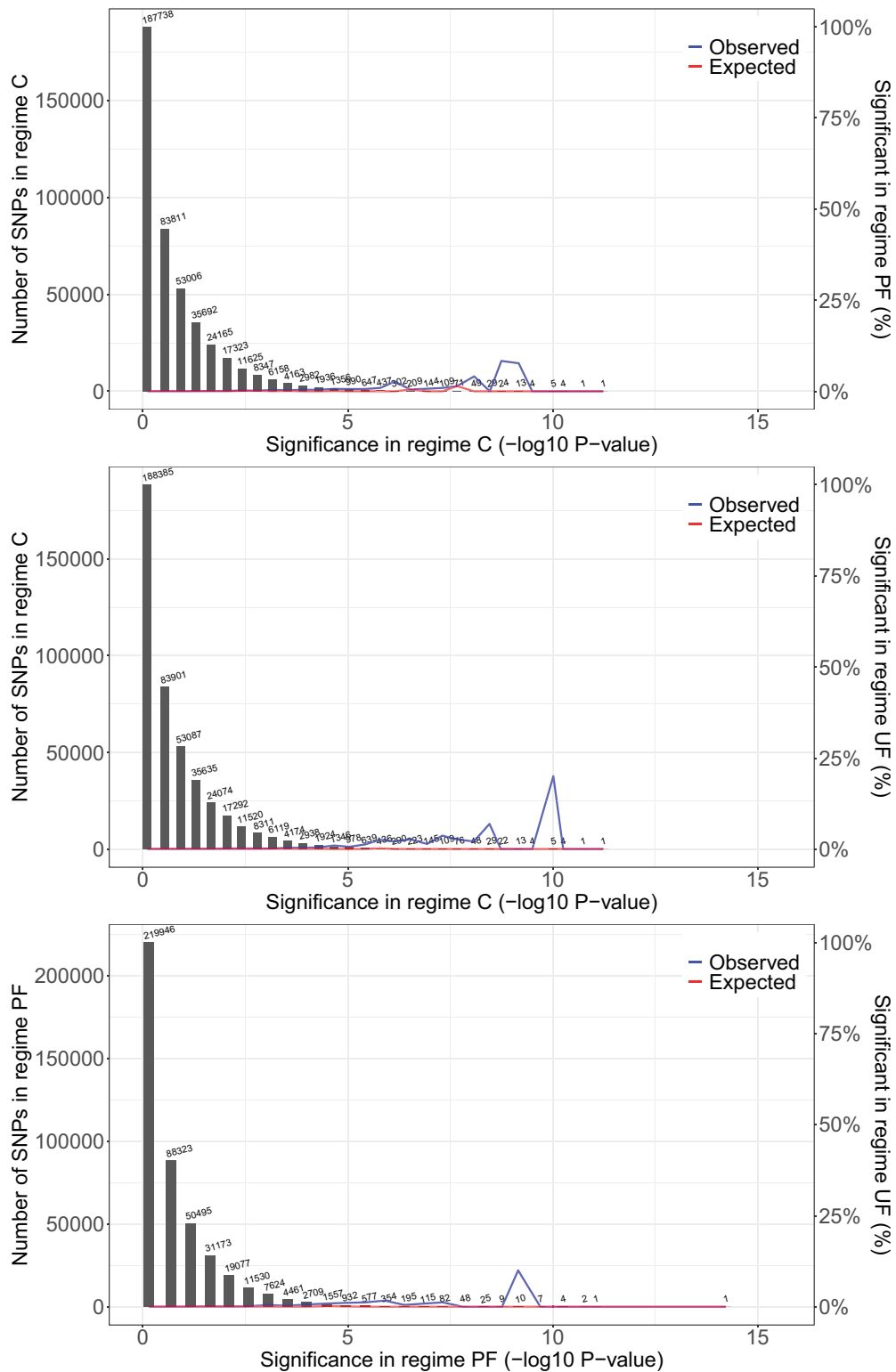
FIGURE 3 | Pairwise overlap of significant SNPs among thermal regimes. Plot shows the distribution of SNP significance [-log10(p-values)] in one regime (gray bars), the observed proportion of SNPs that overlap with significant SNPs in the second regime, and the proportion of SNPs with randomized significance in the second regime that overlap (null-expectation). There is a consistent signal of overlap of SNPs with low p-values (in a small number of SNPs) in all pairwise comparisons. Thus, of the few SNPs with low p-values [high -log10(p)] in one selection regime a larger proportion than expected by chance also have low p-values in the other selection regimes. Only SNPs from chromosome arm 2L are presented here. Results are consistent across chromosomes (see Supplementary Figure 3 ).
