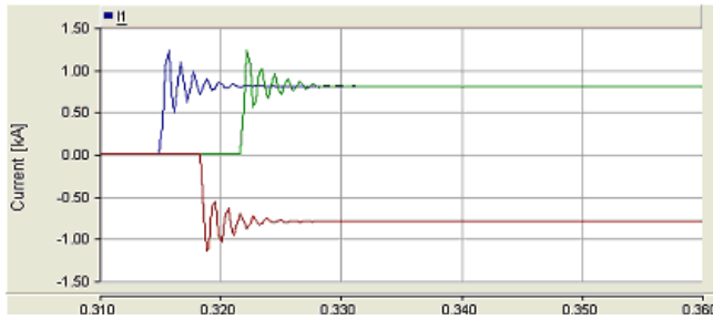
Fig. 11 Circuit Breaker operating in single-pole mode
