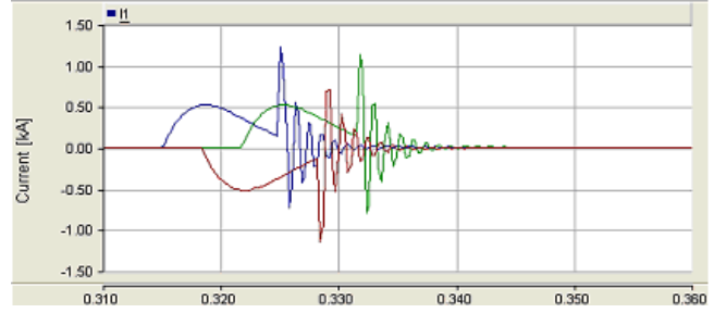
Fig. 13 Simulation of the cable energizing, for a circuit breaker operating in single-pole mode and using pre-insertion resistor
