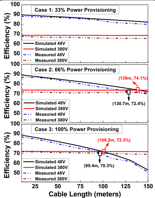
Figure 7. Efficiency variation with conductor length (inter-house distance) variation.
