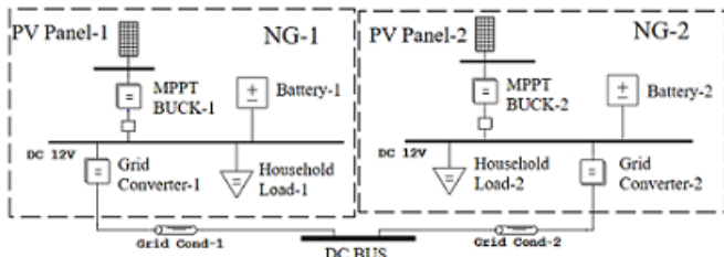
Figure 6. eTap Simulation setup for DGDSA microgrid
