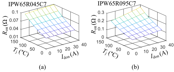
Fig. 9. The built thermal dependent on-state resistance R_{on} with junction temperature T_j and continuous on-state drain current I_{don} as variables. These fitting curves are based on the data extracted from datasheets. Examples (a) IPW65R045C7 and (b) IPW65R095C7.
