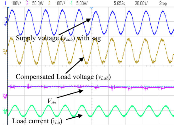
(b) X-axis- 20 \mu sec/div, Y-axis Ch-1,3: 100V/div, Ch-2: 50V/div, Ch-4: 5A/div.
