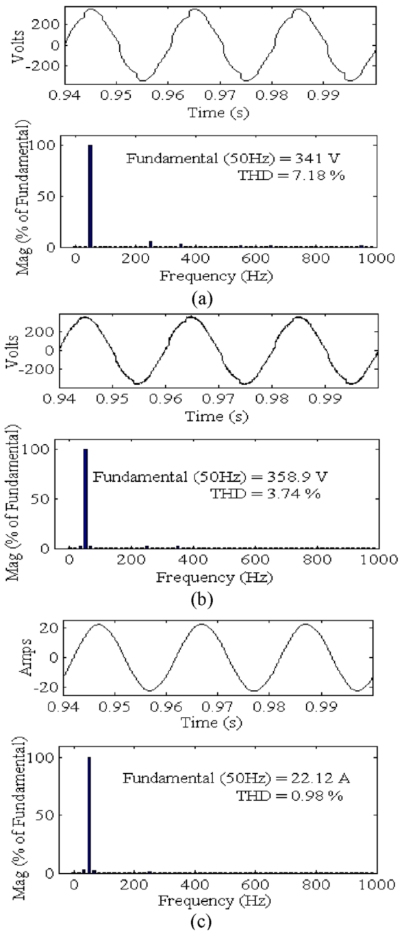
FIGURE 6 Harmonics study of DVR during distortions in supply voltage (a) supply voltage ( v_{sa} ) of phase 'a' and its THD, (b) load voltage ( v_{La} ) of phase 'a' and its THD, and (c) load current ( i_{La} ) of phase 'a' and its THD
