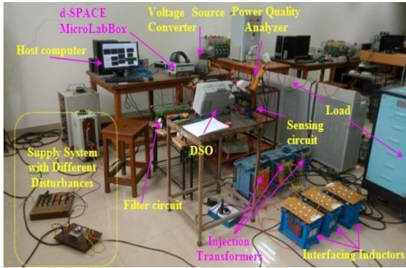
FIGURE 7 Dynamic voltage restorer hardware setup
