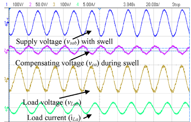
(c) X-axis- 50 \mu sec/div, Y-axis Ch-1,3: 100V/div, Ch-2: 50V/div, Ch-4: 5A/div.
