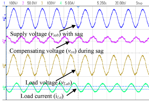
(a) X-axis- 20 \mu .sec/div, Y-axis Ch-1, 3: 100V/div, Ch-2: 50V/div, Ch-4: 5A/div.
