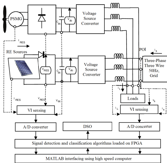
FIGURE 6. General hardware structure of PQ monitoring with RE penetration.
