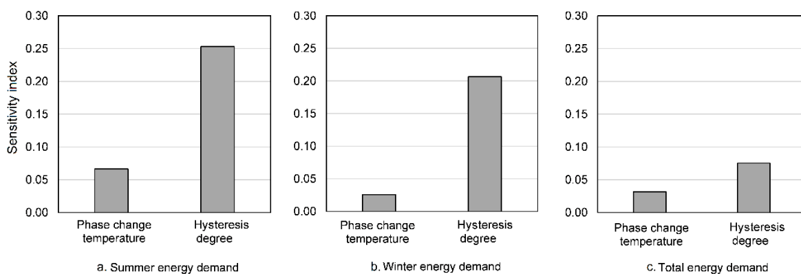
Figure 13. The sensitivity index of phase change temperature and hysteresis degree on the HVAC energy demand: (a) the summer energy demand; (b) the winter energy demand; (c) the yearly total energy demand.
