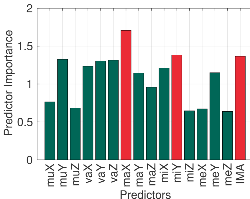
Figure 2. Feature importance in Stage 1, for features mean (mu), variance (va), maximum (ma), minimum (mi), and median (me). X,Y,Z correspond to the respective axis.
