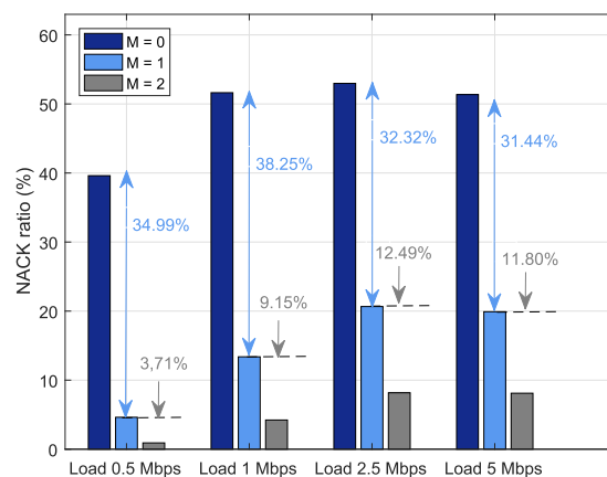
FIGURE 6. Negative acknowledgement ratio for M = 0 , i.e. baseline assumptions, M = 1 and M = 2 for 4 different system loads.
