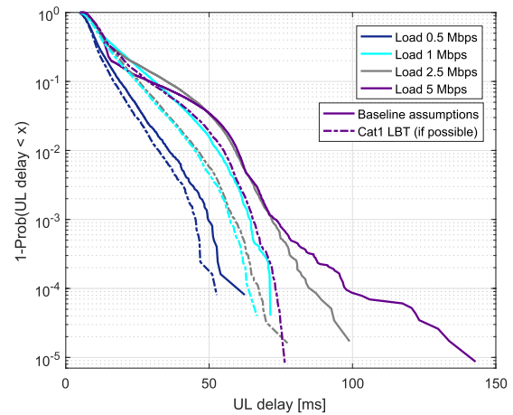
FIGURE 11. CCDF of the delay per packet in uplink. Solid lines represent baseline assumptions while dotted lines show the delay when Cat1 LBT is considered.
