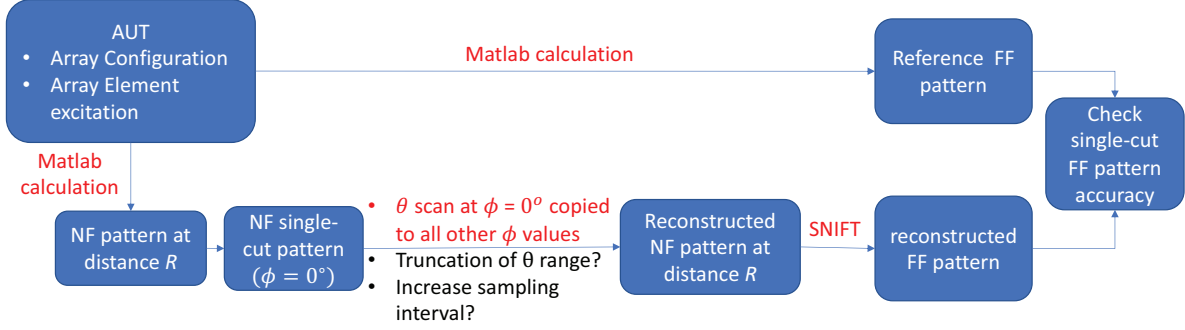
Fig. 4. The proposed simulation framework to investigate the single-cut FF pattern reconstruction accuracy.
