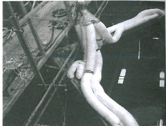
Figure 1 - Picture showing the OWC device, in the preliminary tests moored with a spring board
