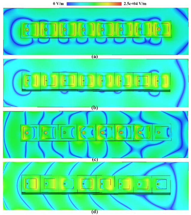
FIGURE 7. E-field distribution of the E-plane arrays with Ant. 1 and the proposed antenna as array elements: (a) and (c) are Ant. 1 at 0° and 60°, respectively; (b) and (d) are the proposed antenna at 0° and 60°, respectively.
