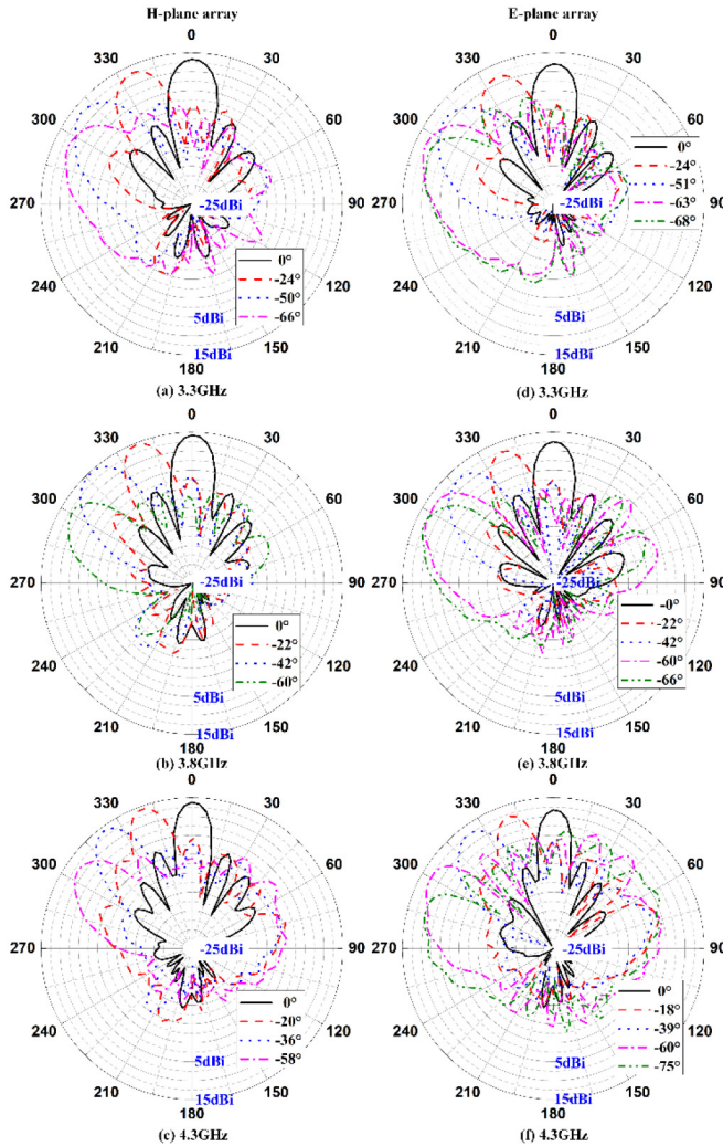
FIGURE 19. Measured scanning patterns of the two arrays.
