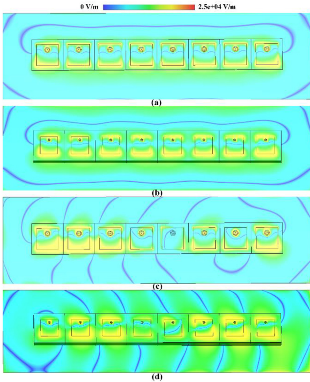
FIGURE 6. E-field distribution of the H-plane array with Ant. 1 and the proposed antenna as array elements: (a) and (c) are Ant. 1 at 0° and 60°, respectively; (b) and (d) are the proposed antenna at 0° and 60°, respectively.
