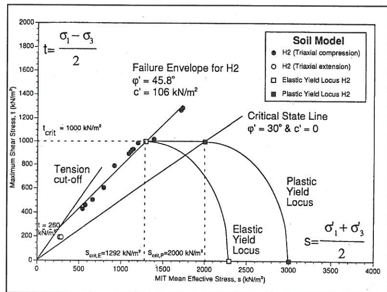
Fig. 2: Principle model for Copenhagen Limestone, [3]
