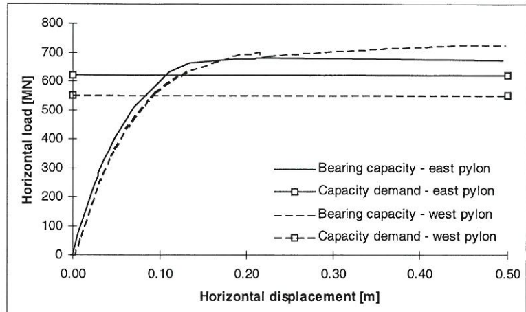
Fig. 5: Load-displacement curve for east and west pylon
