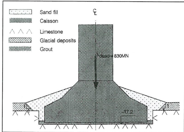
Fig. 1: Geometry and foundation conditions for pylons
