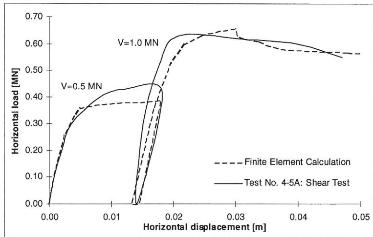
Fig. 4: Calibration to medium scale shear plate test, [3]
