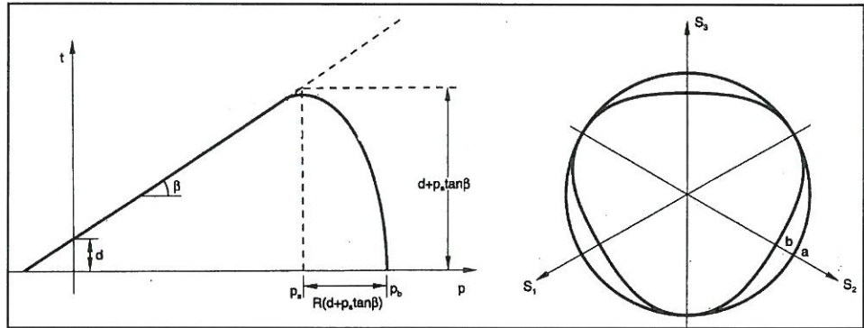
Fig. 3: Drucker-Prager with cap as defined in ABAQUS, [2]
