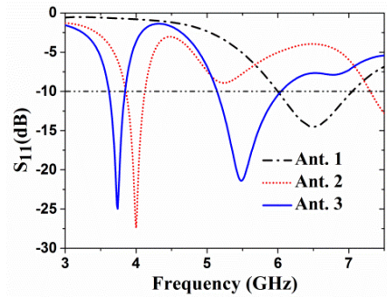
Fig. 3. The reflection coefficients ( S_{11} \leq -10 dB) of the antennas (Ant. 1-3)
