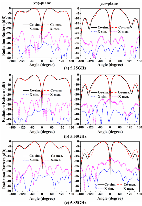
Fig. 9. Simulated and measured normalized radiation patterns of the proposed antenna at 5.25, 5.50 and 5.85GHz
