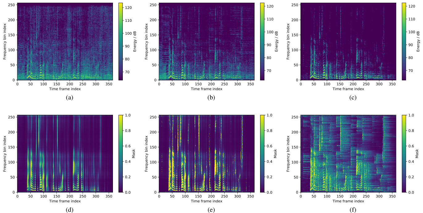
Fig. 5. Example of different noisy and enhanced spectrograms and estimated masks when the REMKF approach is applied to the audio file F05_444C0214_CAF (cafeteria noise, SDR = 7.23 dB) from the CHiME-4 database. (a) Noisy speech spectrogram at the reference channel. (b) Beamformer output spectrogram. (c) Filtered speech signal spectrogram. (d) A priori SPP obtained by the DNN. (e) A posteriori SPP obtained using the REM framework. (f) Kalman gain used in the postfilter.
