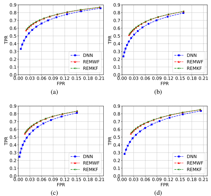
Fig. 3. ROC curves of detectors obtained using the DNN output (a priori SPP) and the a posteriori SPP estimates of the REMWF and REMKF algorithms. The values of the threshold p_{\text{thr}} are chosen between 0.2 and 0.8 with a step of 0.05. The noisy environments analyzed are: (a) bus, (b) cafeteria, (c) pedestrian street and (d) street.
