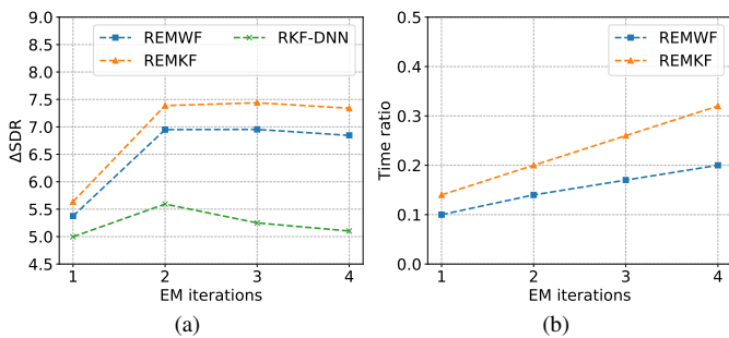
Fig. 4. Performance evaluation of our REMWF and REMKF approaches in terms of the number of EM iterations: (a) Improvements on SDR metric, (b) Time needed to process each second of the noisy speech signal. The analysis of the REMKF using a posteriori SPP estimates directly obtained from the DNN (RKF-DNN) is also included.
