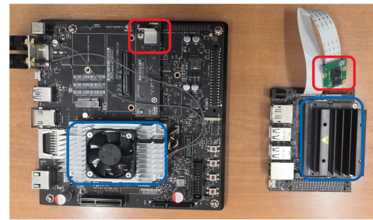
FIGURE 3. The proposed solution: (a) block scheme; (b) the embedded systems employed in the tests. In (b) Jetson TX2 is the device on the left, Jetson Nano is the device on the right. Red rectangles enclose the cameras; blue rectangles enclose the embedded devices hidden by the cooling systems of the development boards.
