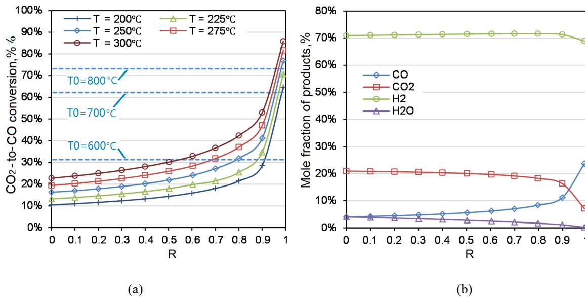
Figure 3. (a) Equilibrium CO 2 -to-CO conversion at different temperatures and R values. (b). The equilibrium composition for the RWGS process at 250°C and different R values.
