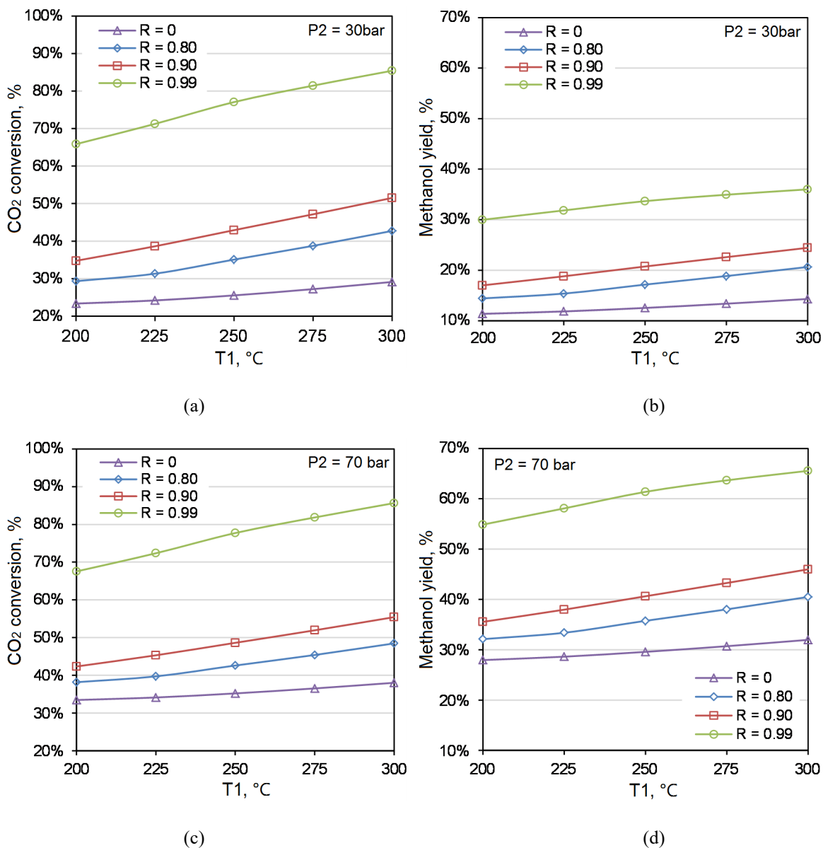
Figure 5. Equilibrium CO_2 conversion (left column) and methanol yield (right column) for the CAMERE process at different T1 and R values (for the RWGS part) and P2 for the MeOH synthesis part.
