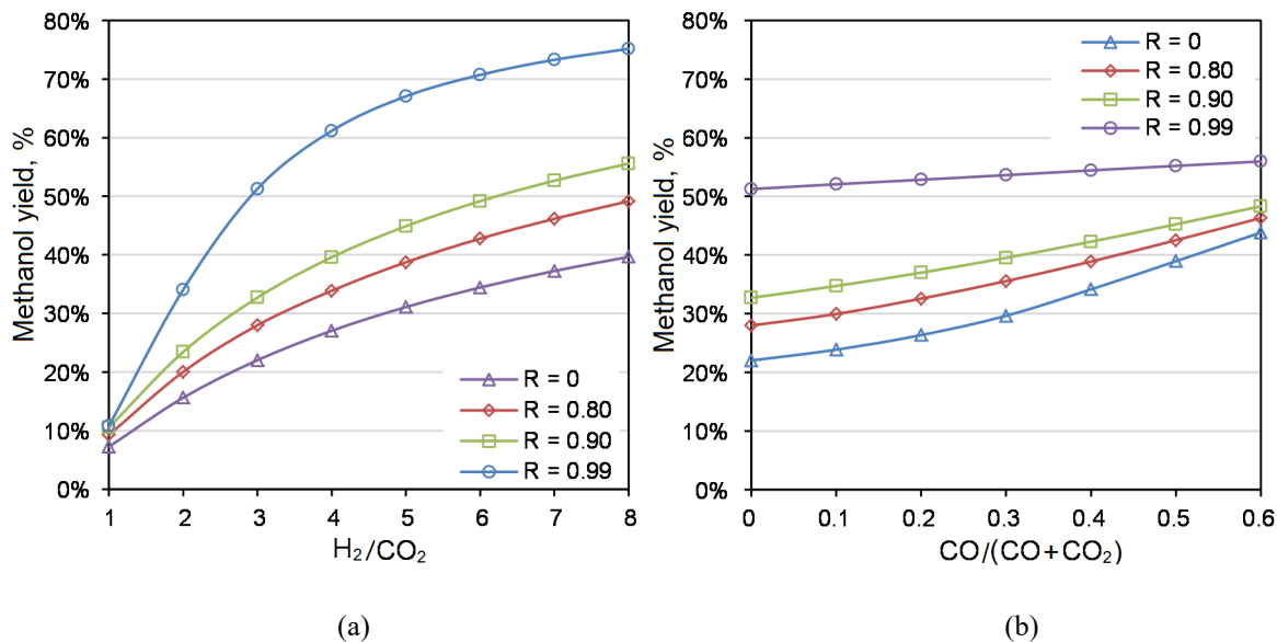
Figure 7. Equilibrium methanol yield at T_1 = T_2 = 250^\circ\text{C} , P_2 = 50 bar and different R values, (a) \text{H}_2/\text{CO}_2 ratios and (b) \text{CO}/(\text{CO}+\text{CO}_2) ratios in the feed gas.
