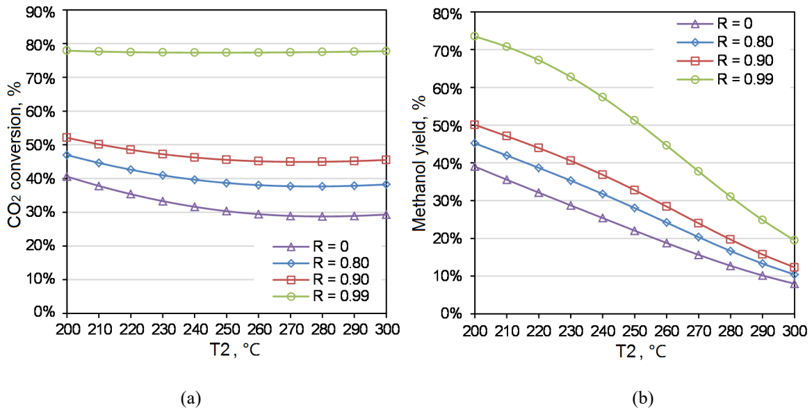
Figure 6. Equilibrium (a) CO 2 conversion and (b) methanol yield at T_1 = 250^\circ\text{C} , P_2 = 50 bar and different T_2 and R values.
