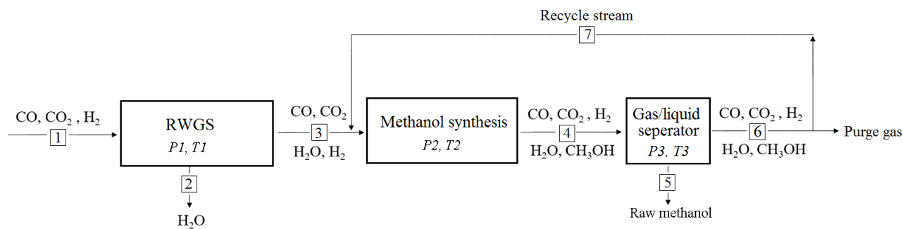
Figure 8. Block scheme of the CAMERE process with ISWR and the recycle stream.
