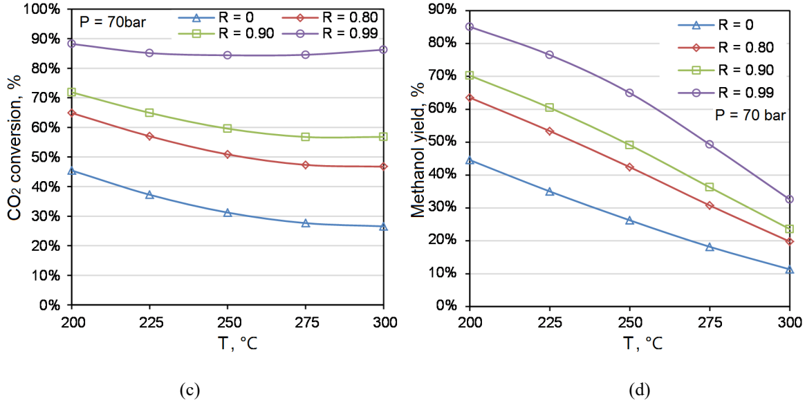
Figure 11. Equilibrium CO 2 conversion (left column) and methanol yield (right column) for the CTM process under the conditions with H 2 /CO 2 = 3 (feed gas), T = 200 – 300 °C, P = 30 – 70 bar and R = 0 – 0.99.
