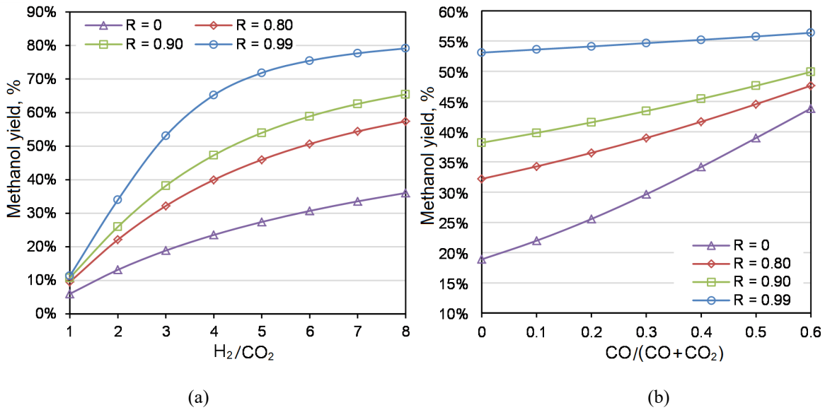
Figure 12. Equilibrium methanol yield at T = 250°C, P = 50 bar and different R values, (a) H 2 /CO 2 ratios and (b) CO/(CO+CO 2 ) ratios in the feed gas for the CTM process.
