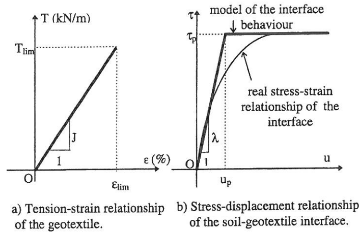
Fig. 9. Tensile and friction behaviour of the inclusion.
