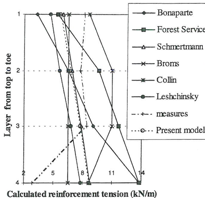
Fig. 19. Reinforced tension calculated for RMC wall configuration.
