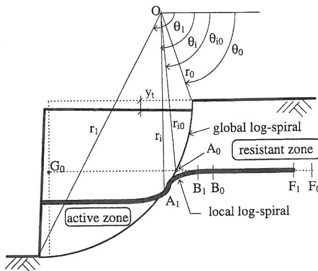
Fig. 10. Displacement compatibility.
