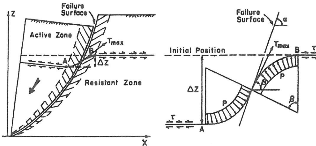
Fig. 2. Anchored membrane concept for geotextile reinforcement (Gourc et al., 1986).
