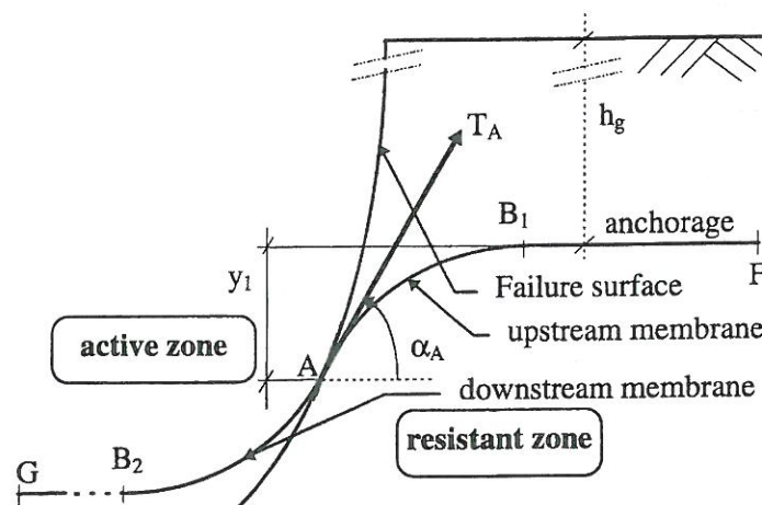
Fig. 3. Anchored membrane. Notations.
