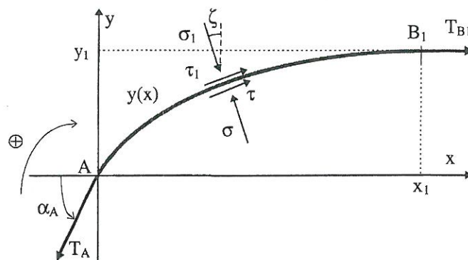
Fig. 4. Free body diagram of upstream membrane AB_1 .
