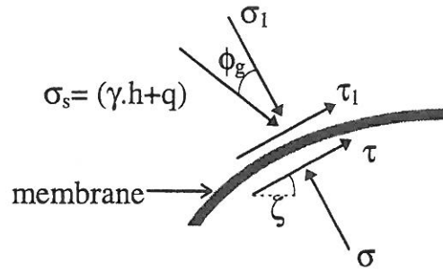
Fig. 5. Model 1 for \sigma_1 distribution.
