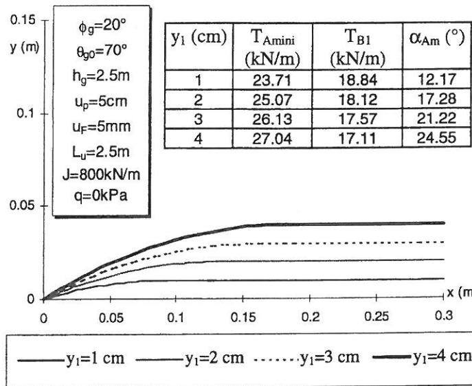
Fig. 16. Critical positions of the membrane for y_1 = 1-4 cm (model 4).
