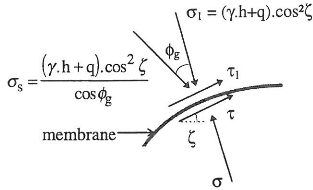
Fig. 6. Model 2 for \sigma_1 distribution.
