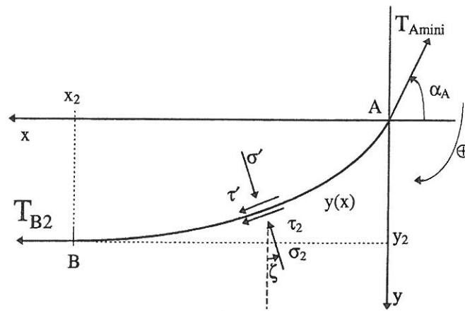
Fig. 8. Free body diagram of downstream membrane AB_2 .
