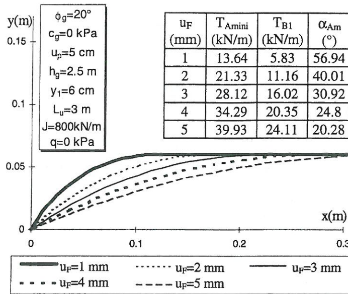
Fig. 14. Critical positions of the membrane for u_F = 1-5 mm (Model 4).
