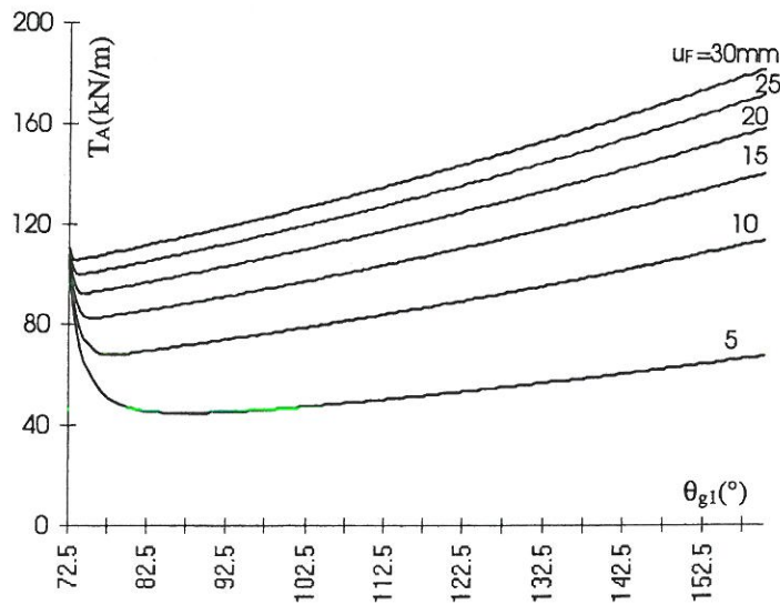
Fig. 13. Variation of T_A versus \theta_{g1} for u_F = 5\text{--}30 \text{ mm} (Model 4).
