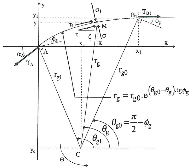
Fig. 7. Shape of the upstream membrane from the present variational analysis.
