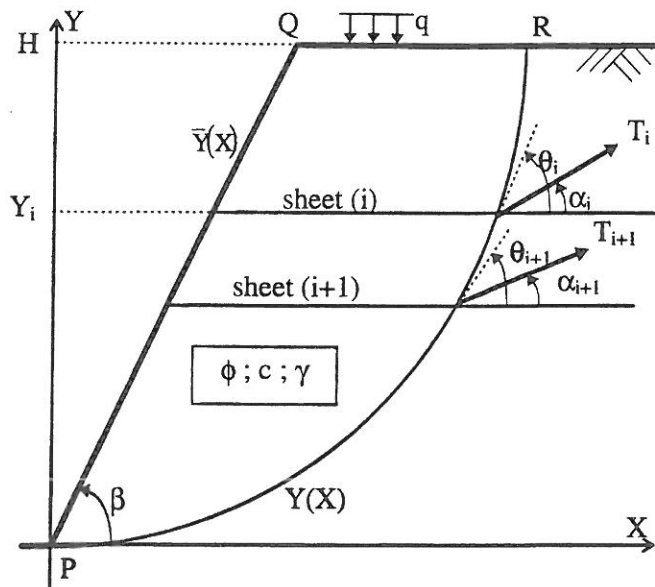
Fig. 1. Geotextile reinforced slope stability analysis.
