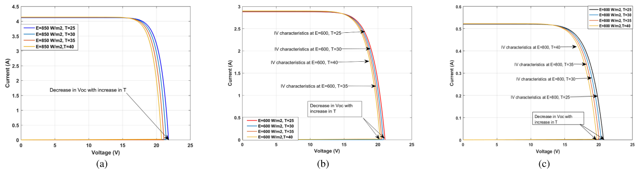
FIGURE 7. I-V characteristics at variable temperature levels while keeping irradiance constant. (a) Plant 1. (b) Plant 2. (c) Plant 3.
