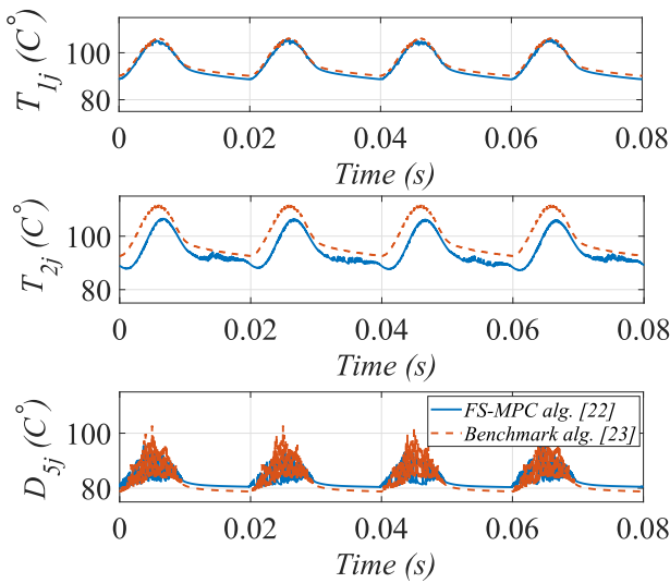
(c) Device junction temperatures cycles.
