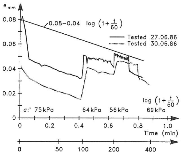
Fig. 11. Block 4, side 5-6. Calculated variations in e against \log(1 + \frac{t}{60}) .
