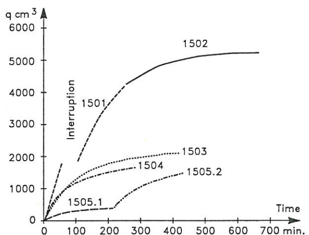
Fig. 6. Block 15 (75x75x75cm 3 ). Results of flow tests.
