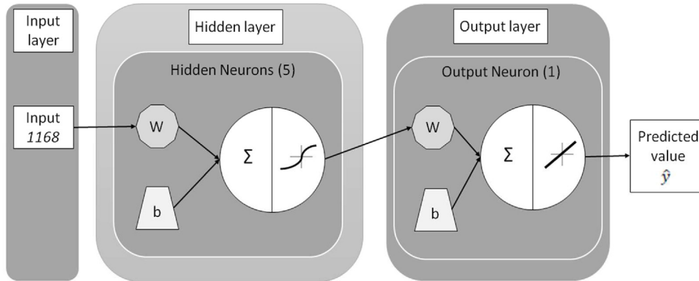
Fig. 1. SPFFNN PP forecaster's layout.
