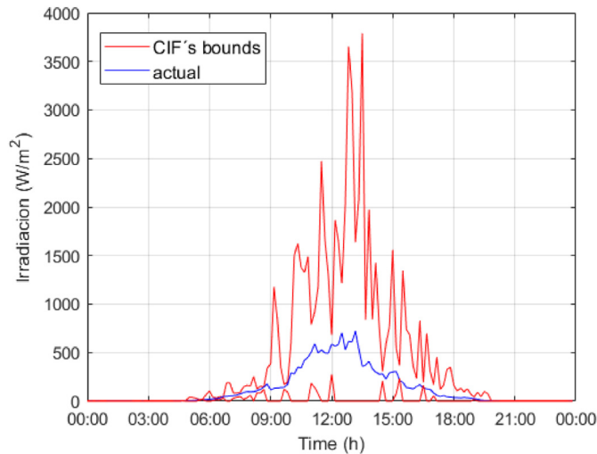
Fig. 8. Forecasted intervals and actual solar irradiation evolution for June 15, 2017 (cloudy day, PICP_{0.05} = 95.83 and SSN_{0.05} = 4.15 ).
