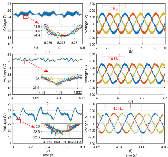
FIGURE 15. Experimental results. (a), (c) and (e) show the 3x3-MMSC submodule-capacitor voltages for the cases f_o = 1, 10 and 45 Hz, respectively. (b), (d) and (f) show the 3x3-MMSC load voltages ( v_{oabc} ) for the cases f_o = 1, 10 and 45 Hz, respectively.
