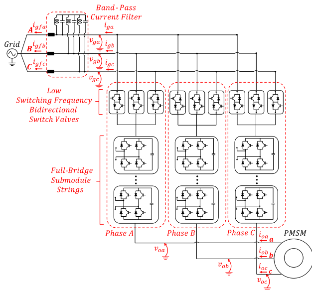
FIGURE 4. 3x3-MMSC topology.
