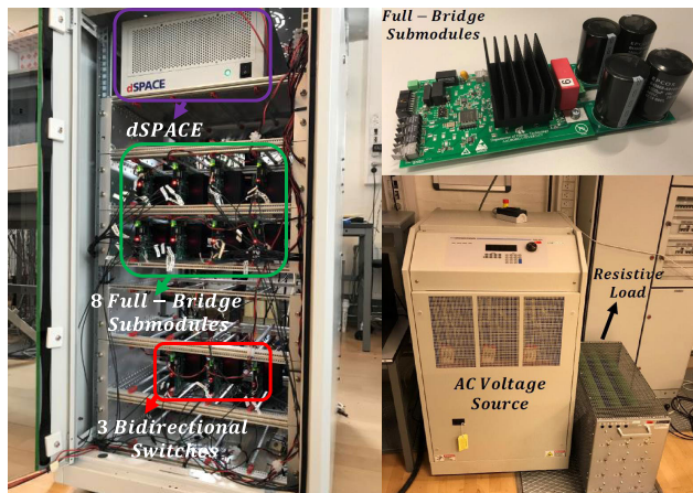
FIGURE 14. 3x3-MMSC test setup.
