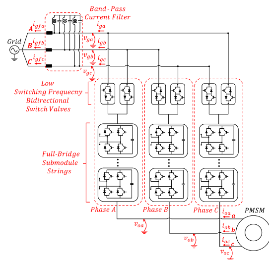
FIGURE 3. MMSC topology.
