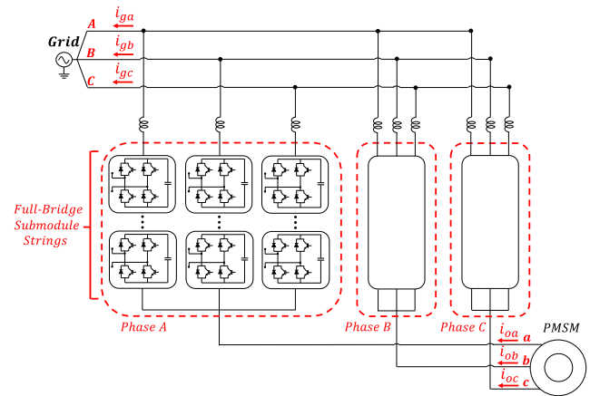
FIGURE 2. M^3C topology.
