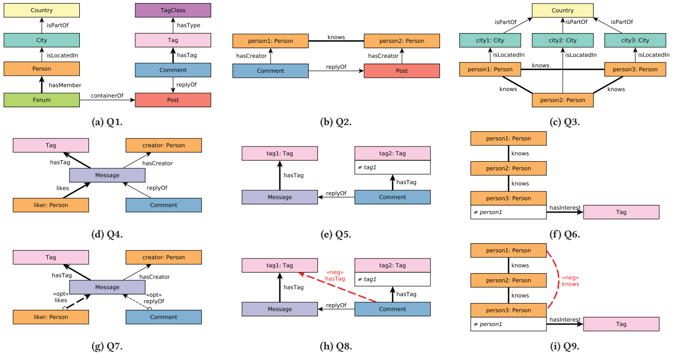
Figure 3: Visualization of the queries. Regular edges (joins) are denoted with solid black lines. Negative edges (antijoins) are denoted with dashed red lines and the «neg» keyword. Optional edges (left outer joins) are denoted with dashed black lines, the «opt» keyword, and the circle symbol \circ at the optional end of the edge. Thicker lines denote edge labels with many-to-many cardinality.
