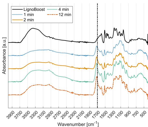
Figure 6: ATR spectra of the ASO, with the 1700 cm -1 carboxylic wave number marked by the dashed black line.
