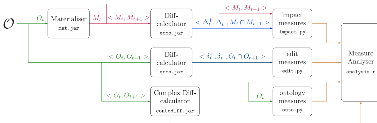
Fig. 2. Calculation Pipeline.
