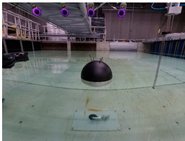
Figure 10. Test setup in the wave basin: center—half-submerged sphere model; background—motion capture cameras (stroboscopes in purple); right—wave gauge (number 3).
