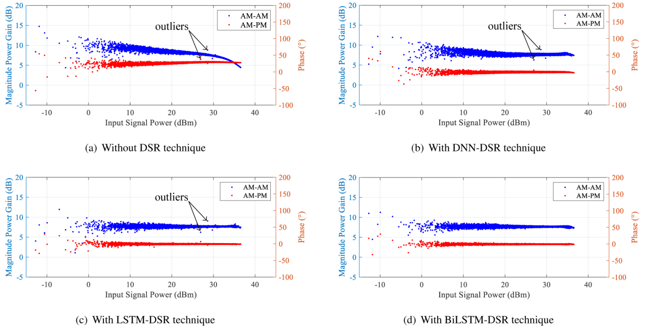
FIGURE 10. AM-AM and AM-PM curves with different DSR techniques for the 10MHz OFDM signal. (a) Without DSR technique, (b) with DNN-DSR technique, (c) with LSTM-DSR technique, (d) with the proposed BiLSTM-DSR technique.
