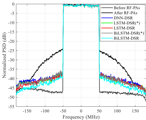
(b) 100MHz bandwidth and 11.69 dB PAPR signal.
