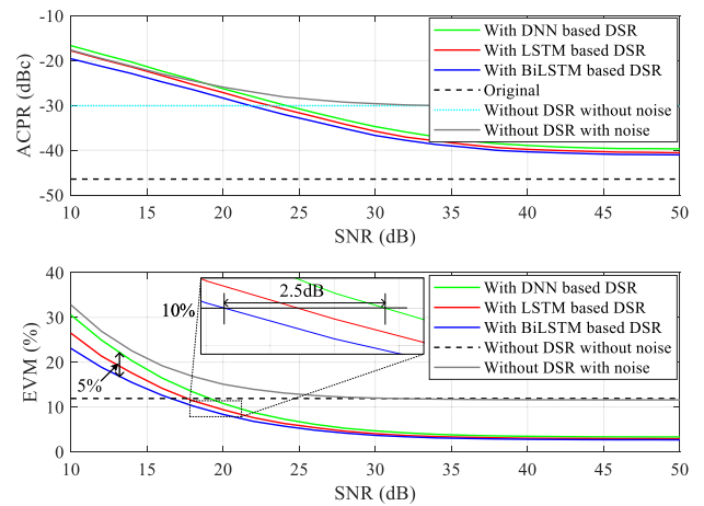
(b) 100MHz bandwidth and 11.69 dB PAPR signal.
