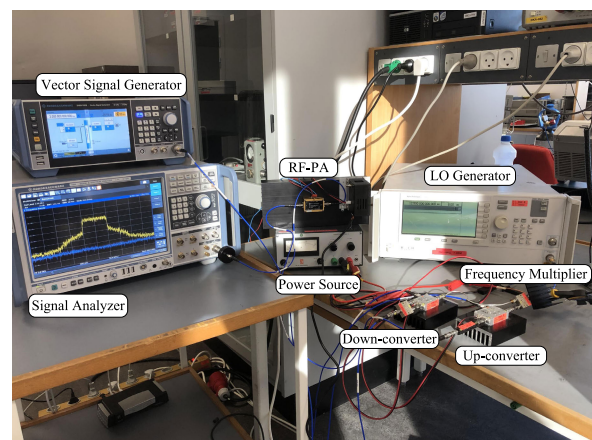
FIGURE 9. Photograph of the measurement setup.
