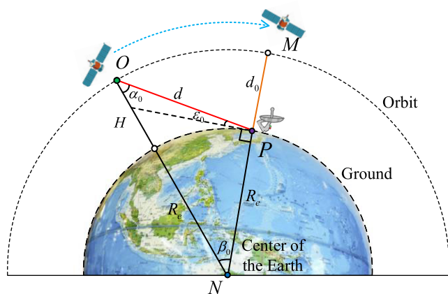
FIGURE 2. Geometry graph of the satellite-to-ground data transmission link.
