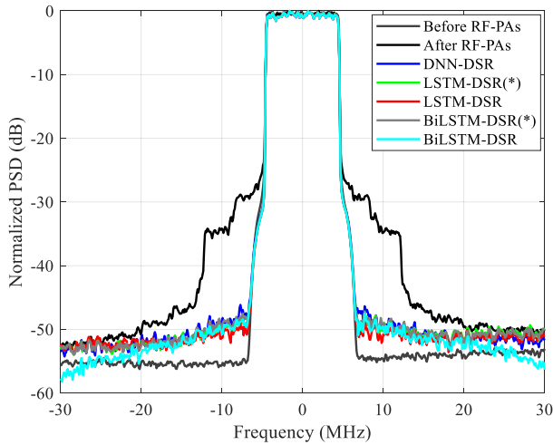
(a) 10MHz bandwidth and 10.06 dB PAPR signal.
