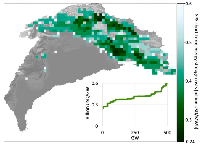
Figure 5. Short-term energy storage costs with SPHS plants.
