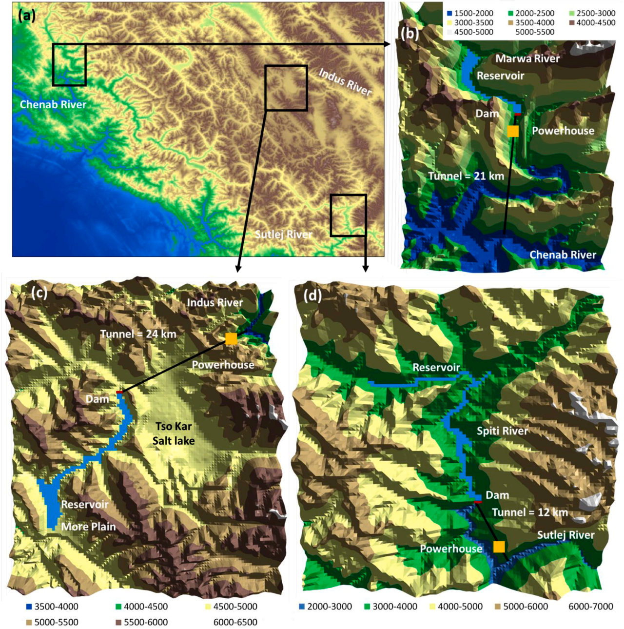
Figure 3. Description of the proposed SPHS plants. (a) Topography of the upper Indus basin, (b) Marwa, (c) More and (d) Spiti SPHS plants.
