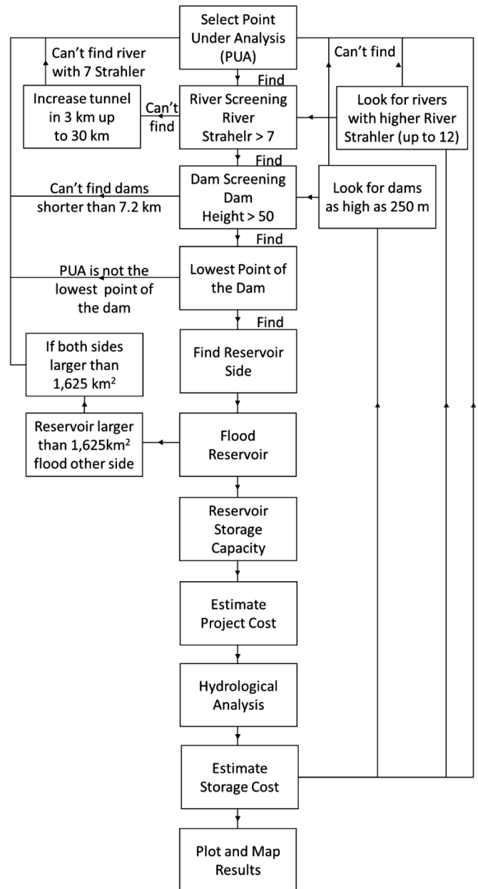
Figure 1. Global siting of hydropower and SPHS projects model framework implemented on the Indus basin.
