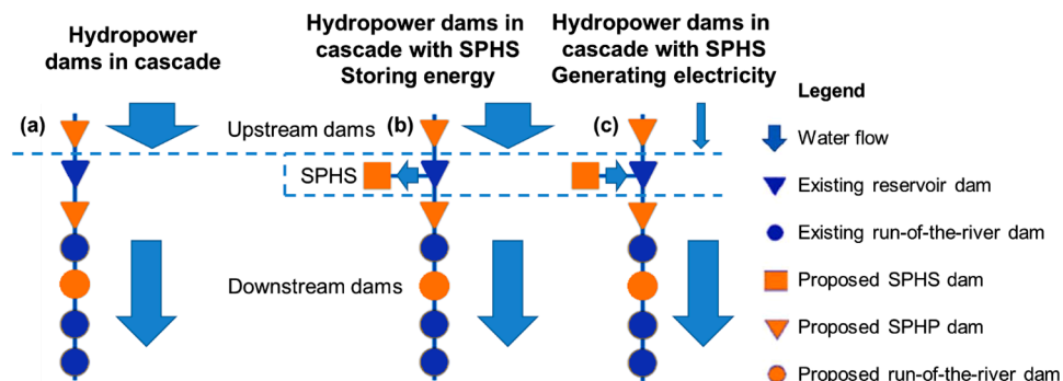
Figure A.10. Operation of (a) conventional hydroelectric plants (b) SPHS during periods of high-water availability (c) SPHS during periods of low water availability. Note that the same legend is used in other figures [61].
