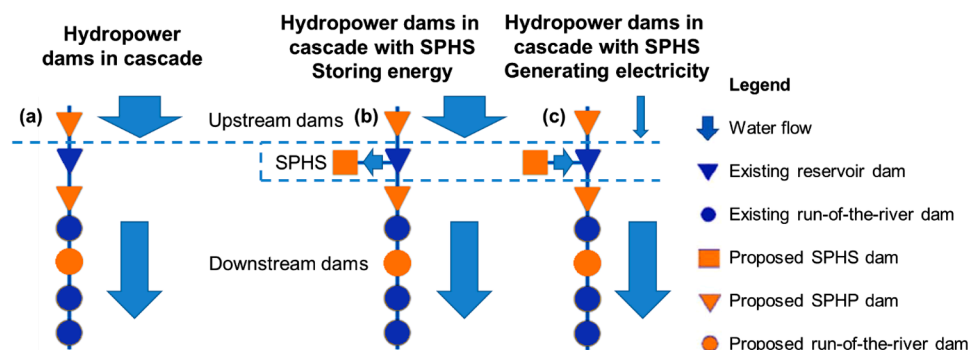
Figure A.10. Operation of (a) conventional hydroelectric plants (b) SPHS during periods of high-water availability (c) SPHS during periods of low water availability. Note that the same legend is used in other figures [61].
