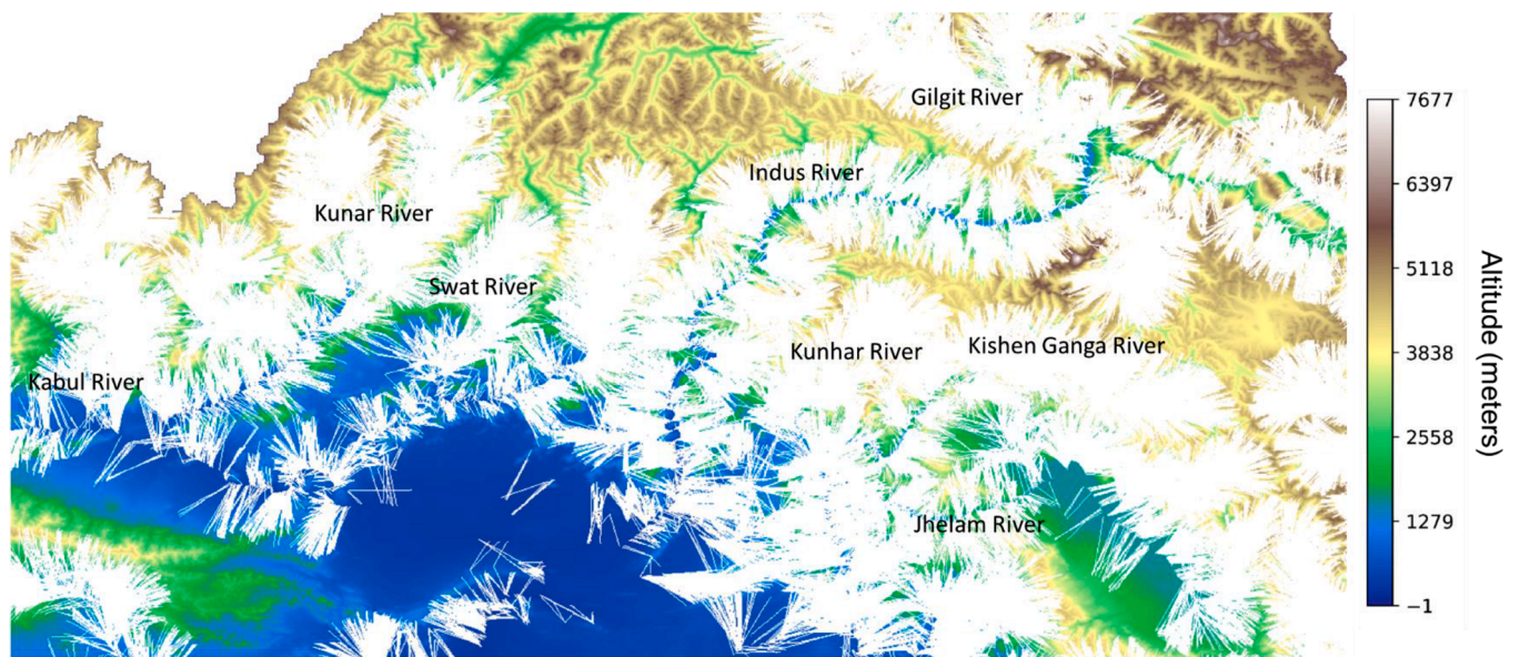
Figure C.14. Seasonal pumped hydropower storage plants developed by the model in the Indus basin, where the tunnels are represented in white.
