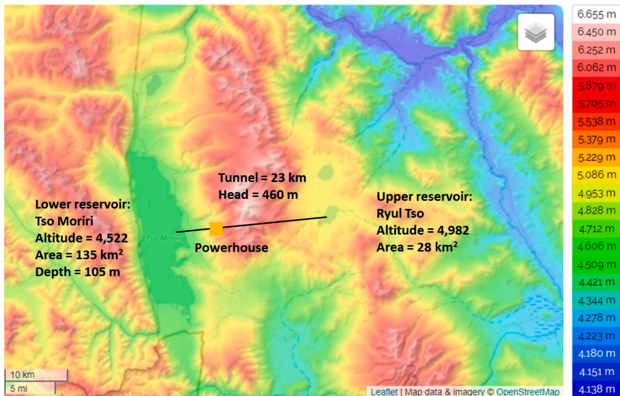
Figure 9. Possible closed loop project with existing salty lakes [52].
