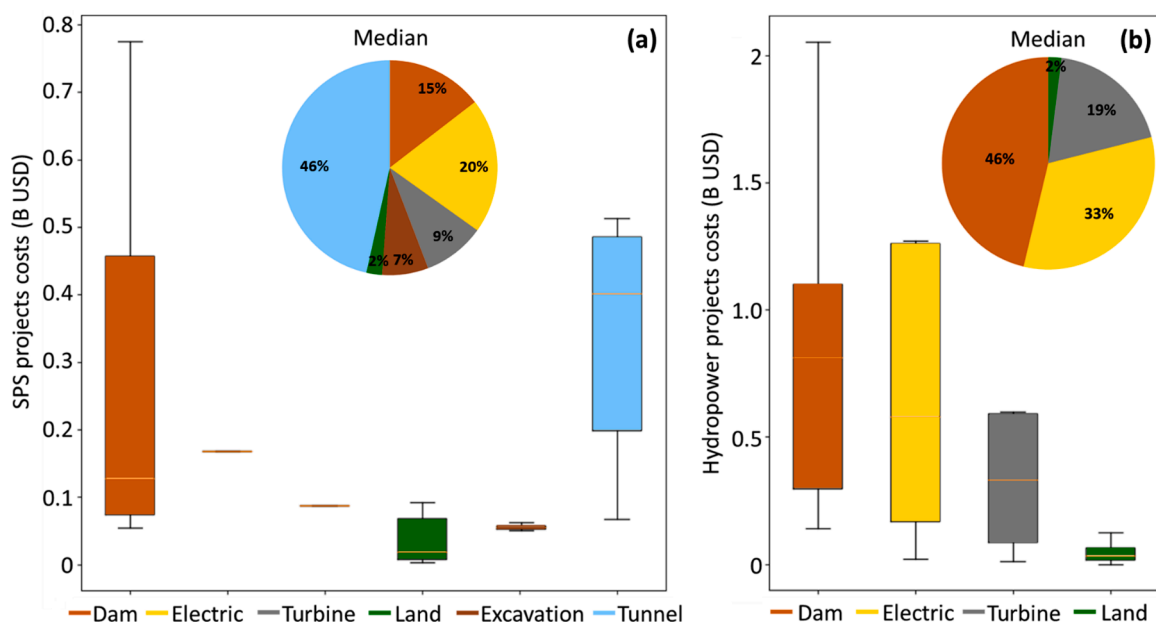
Figure 6. (a) Cost of SPHS projects with long-term energy storage, (b) cost of hydropower projects with generation. The range shows the values between 5% and 95% of the sample data, with the bars for between the first and third quartile. The line on each bar shows the median of each range.
