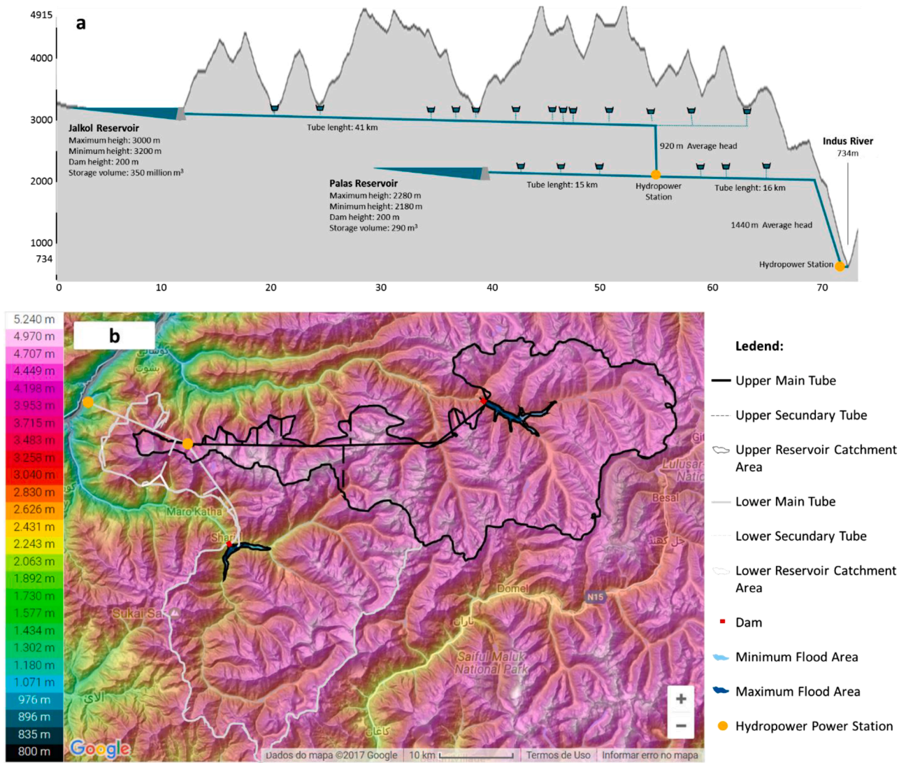
Figure 7. Proposal of a combination of two SPHS system with one connection to the Indus River.
