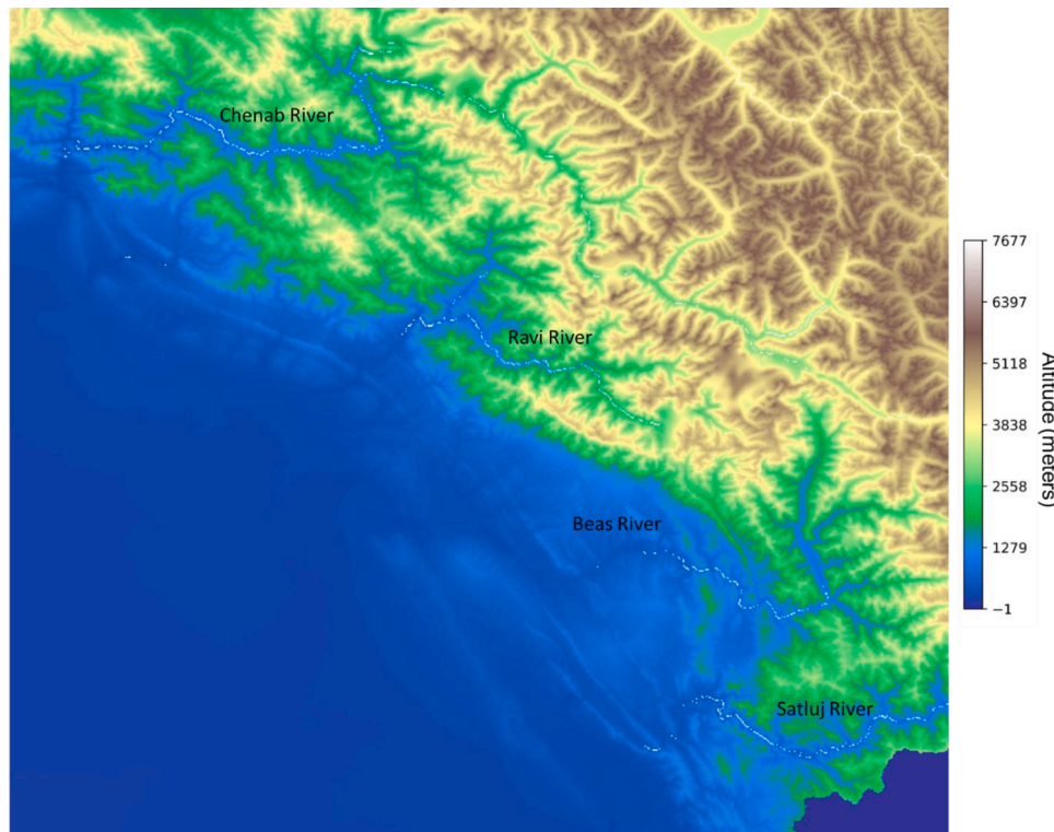
Figure C.12. Hydropower projects investigated on the Chenab and Satluj river basins. The white dots are the locations where the dams were proposed.
