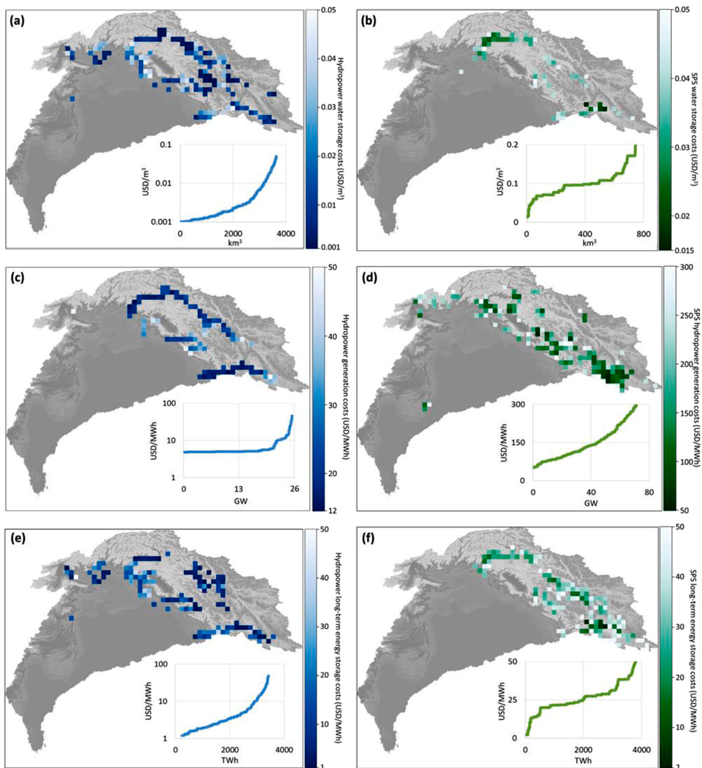
Figure 2. Water storage costs with (a) hydropower plants and (b) SPHS plants; hydropower generation costs with (c) hydropower plants and (d) SPHS plants; long-term energy storage costs (e) hydropower plants and (f) SPHS plants.
