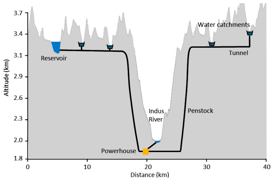
Figure 8. SPHS system with the powerhouse connected to reservoir and catchments on both sides of the river.
