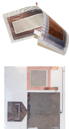
Figure 2: Top: SATURN - thin and flexible self-powered microphone [4] , Bottom: ZEUSSS : Zero-energy Ubiquitous Sound Sensing Surface [3].
