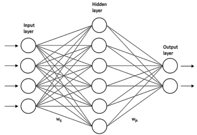
Fig. 3. ANN structure [29]
