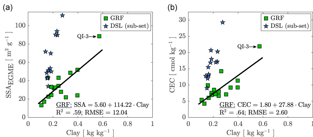
FIGURE 5 (a) Specific surface area ( \text{SSA}_{\text{EGME}} ) ( \text{m}^2 \text{g}^{-1} ) and (b) cation exchange capacity (CEC) ( \text{cmol kg}^{-1} ) of the glacial rock flours (GRFs) as a function of the gravimetric clay. A subset of the Danish soil library dataset (DSL) (13 out of 41 soils) with similar clay and organic matter content was added for reference
