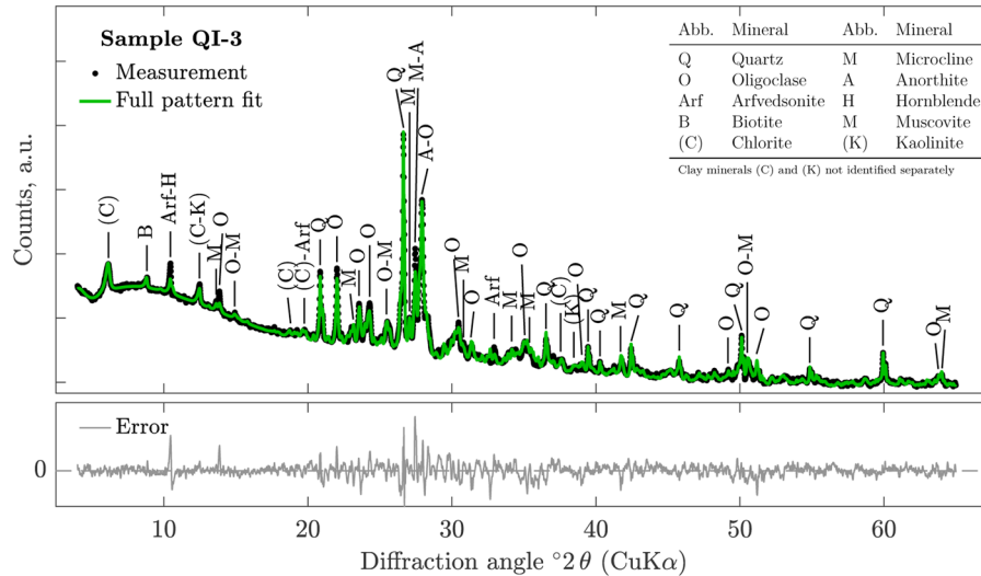
FIGURE 4 Example X-ray diffraction diffractogram for sample Quingua (QI)-3. Counts per second (black dots) and Rietveld fit (green) and the corresponding error (grey) in the bottom subplot. The phyllosilicates chlorite (C) and kaolinite (K) were not identified separately on the <2\text{-}\mu\text{m} fraction, but their potential diffraction peaks were indicated
