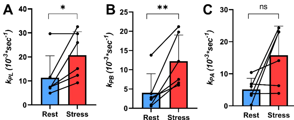
Fig. 5 Conversion rate constants. A–C The mean k_{PL} , k_{PB} and k_{PA} at rest and during stress. The mean k_{PL} increased statistically significantly from 11 \pm 9 * 10^{-3} s^{-1} to 20 \pm 10 * 10^{-3} s^{-1} , p = 0.04 . The mean k_{PB} increased statistically significantly from 4 \pm 4 * 10^{-3} s^{-1} to 12 \pm 7 * 10^{-3} s^{-1} , p = 0.008 . The k_{PA} increased from 5 \pm 3 * 10^{-3} s^{-1} to 16 \pm 9 * 10^{-3} s^{-1} , p = 0.06
