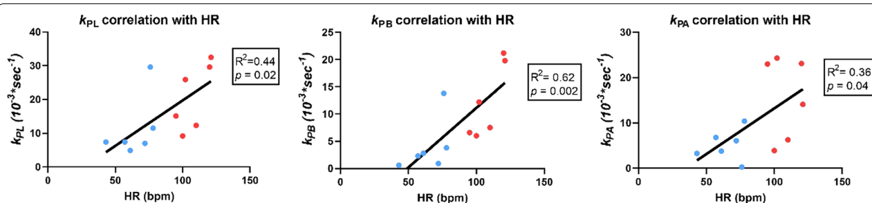
Fig. 6 Conversion rate constants correlation with HR. There was a positive and statistically significant correlation of HR and increase in k_p for both lactate ( p = 0.02 ), bicarbonate ( p = 0.002 ) and alanine ( p = 0.04 ). HR, heart rate
