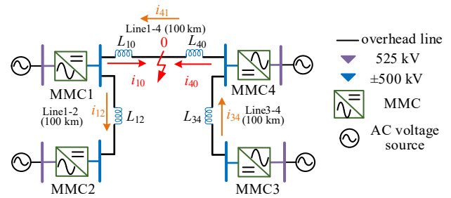
Fig. 3. Topology of HVDC grid.
