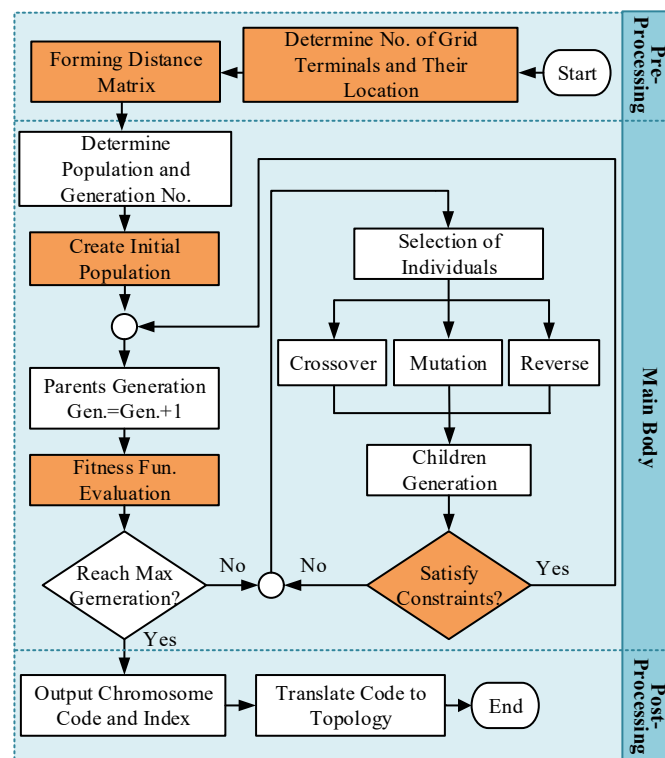
Fig. 9. The procedure of genetic algorithm for topology optimization.
