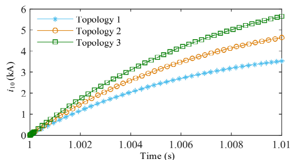
Fig. 8. Curves of i_{10} under three topologies.
