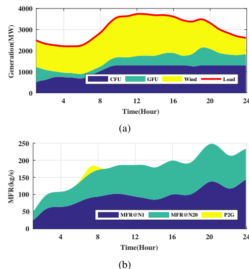
Fig. 10. Optimal schedule of IGPS. (a) Optimal generation schedule. (b) Optimal gas system schedule.
