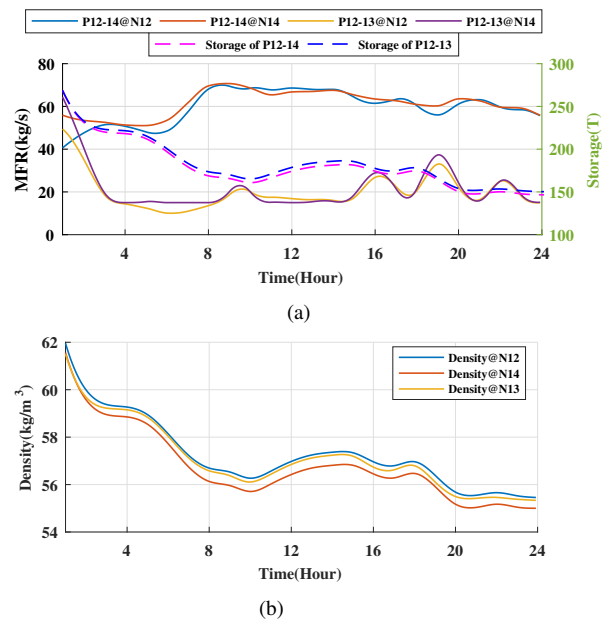
Fig. 12. The dynamic performance of IGPS. (a) The MFR at each end of the pipeline 12-13 and pipeline 12-14, and the storage in both pipelines. (b) The density at each end of the pipeline 12-13 and pipeline 12-14.
