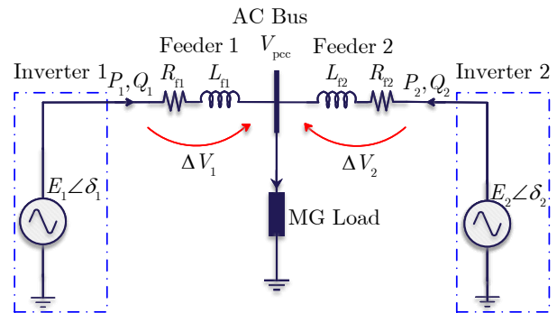
Fig. 1: Equivalent model of the islanded microgrid system consisting of two droop-based inverters.
